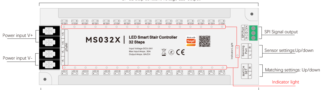
01-16 Step constant voltage LED output
