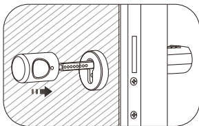
7. Install the rear handle to the fit position.Rear handle screw holes must be aligned with the square bar locating holes
