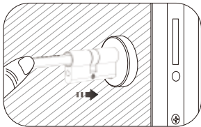
3. Rotating square axle to align the cam with the lock cylinder,install the lock cylinder into the door.
