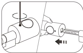
1. Take out the screws and take out the rear handle
