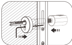
5. Rotating square axle to raise the cam, insert screwdriver into the bottom of lock cylinder.Insert the front handle and adjust it to the fit position.
