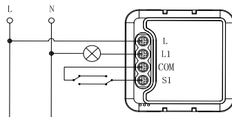
Double Switch
