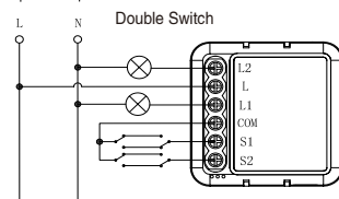
Wiring diagram of fittings(L1 L2 One of them)
