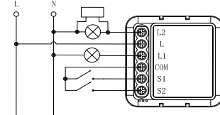
Wiring diagram of fittings(L1 L2 One of them)
