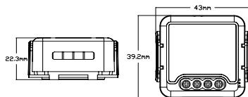
Single Control
