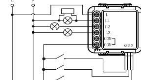
Wiring diagram of fittings(L1 L2 L3 One of them)
