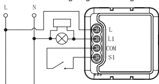
Wiring diagram of fittings
